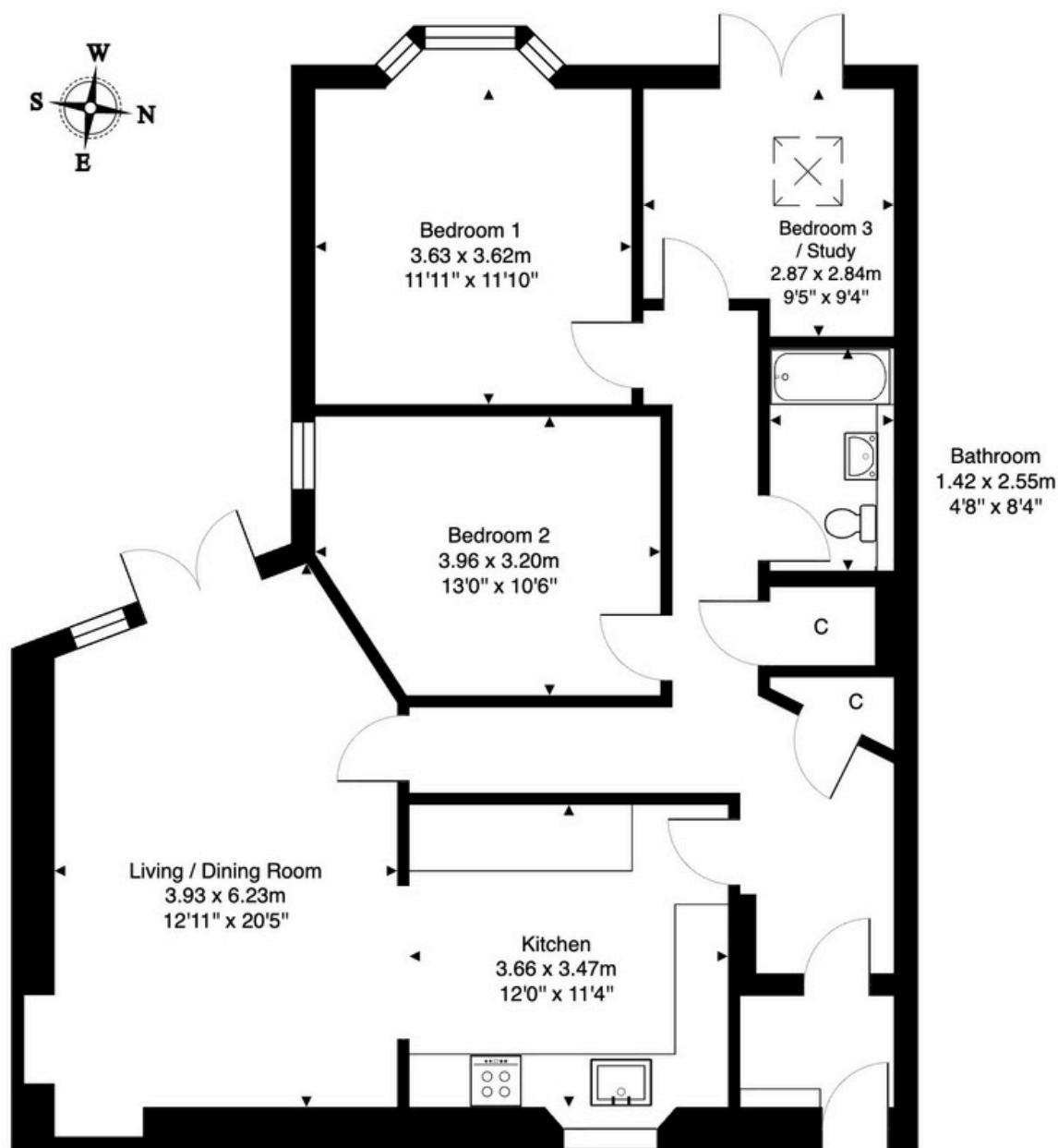
Ground Floor
